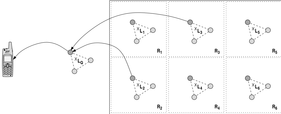
Figure 2: Hierarchical GHT in combination with partial evaluation
