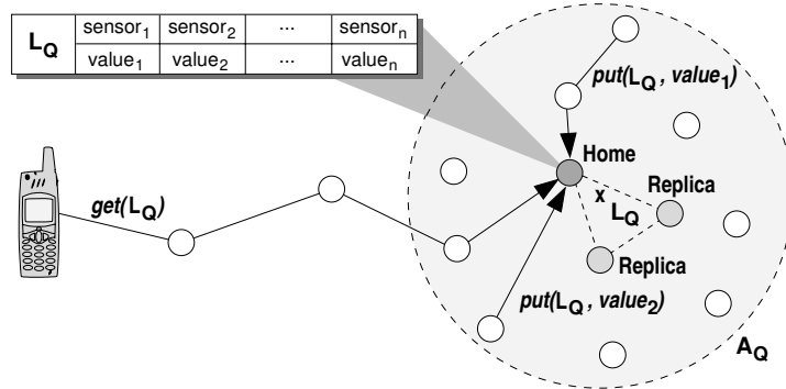
Figure 1: GHT in combination with packet merging
