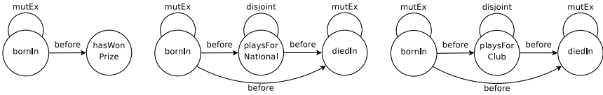
(c) The minimal set \mathcal{G}_M of common subgraphs of G_M^{max} (Figure 2(b)) and G_C (Figure 2(a)) covering all edges of G_C .
