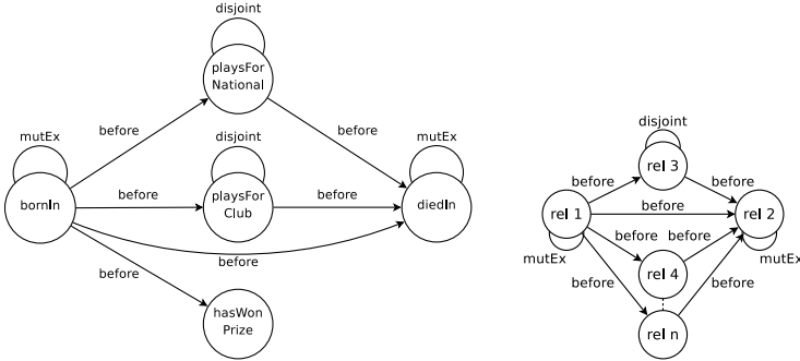
(a) Constraint graph G_C of our running example, where each edge represents one of the constraints depicted in Appendix A. (b) The maximal machine graph G_M^{max} , where n \in \mathbb{N} , n \geq 4 .
