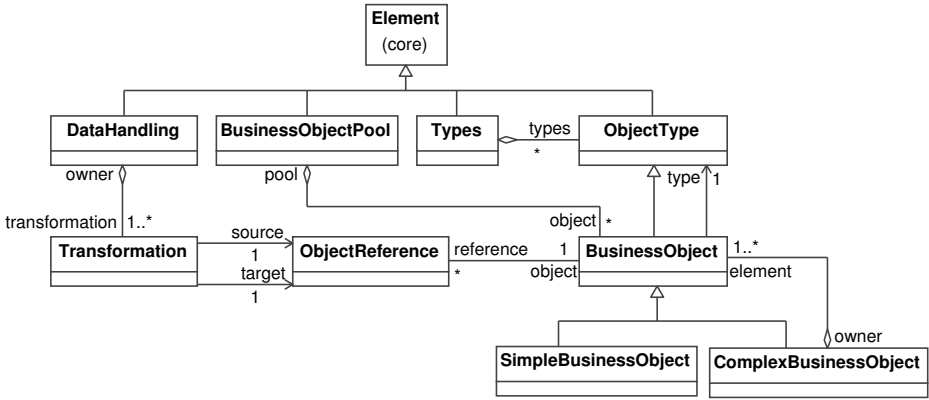
Figure 5: Information view meta-model
