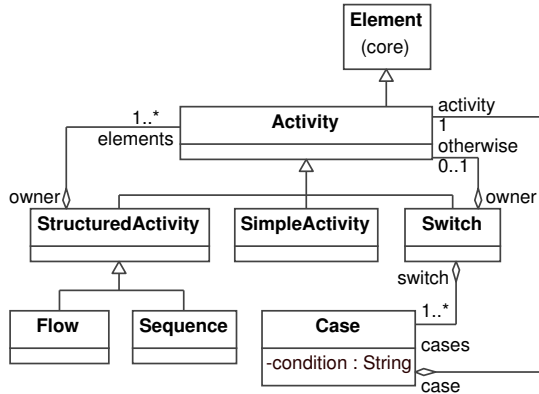
Figure 3: Orchestration view meta-model
