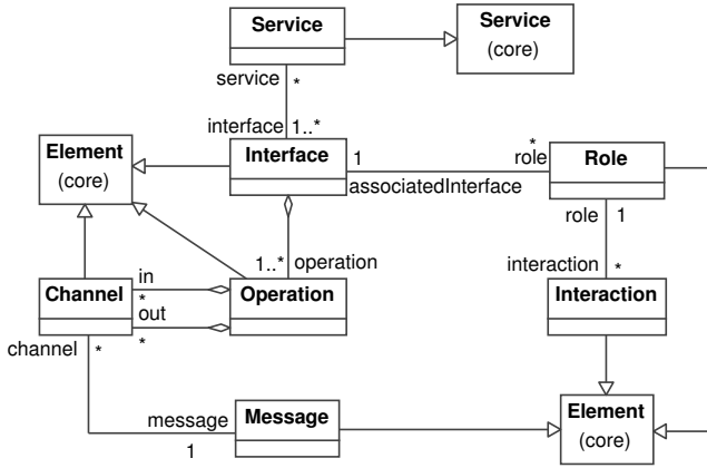
Figure 4: Collaboration view meta-model
