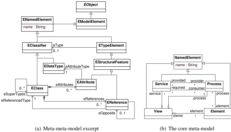
Figure 2: Meta-meta-model and the Core meta-model
