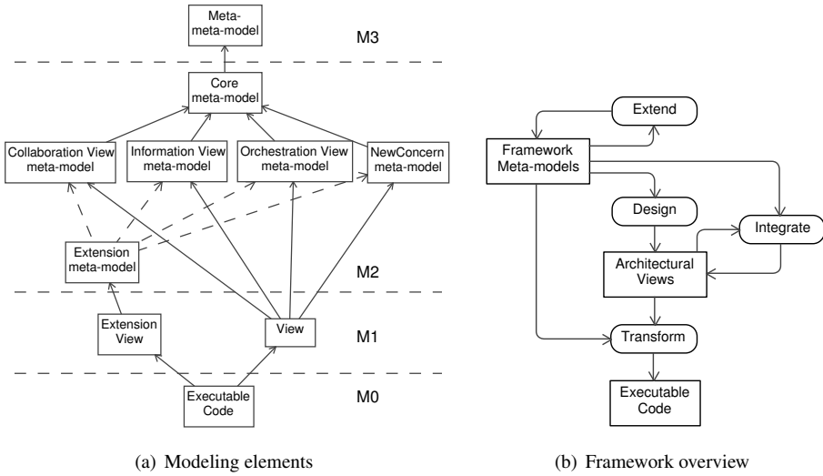
Figure 1: View-based model-driven framework
