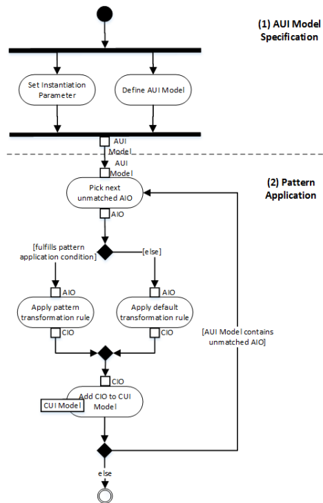
Figure 2: Pattern application workflow.
