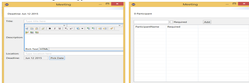
Figure 6: Screenshot excerpts of the generated UI for the calendar management application where different GUI patterns were automatically applied during the transformation process.
