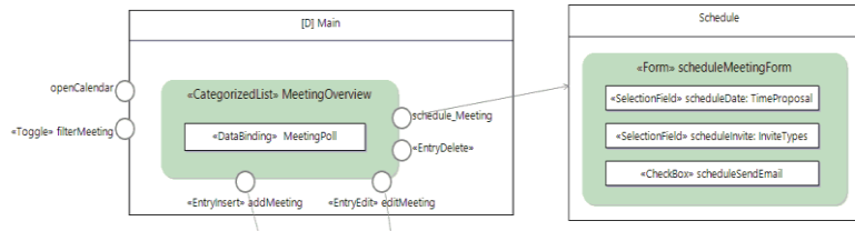
Figure 5: Excerpt of the Calendar Management abstract UI.
