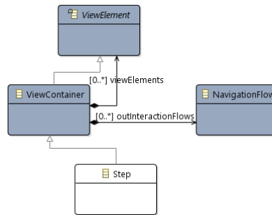
Figure 3: Wizard pattern extension.
