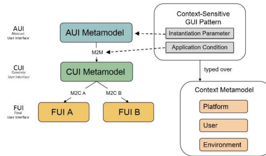
Figure 1: Integration of Context-Sensitive GUI Pattern.
