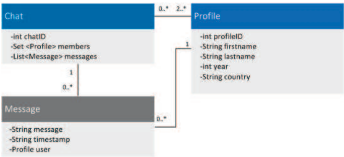
Figure 3: Class diagram for example scenario (extract).
