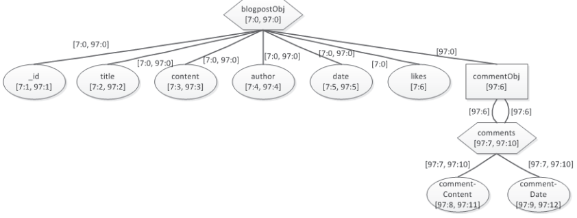
Figure 5: Structure identification graph for the sample entities
