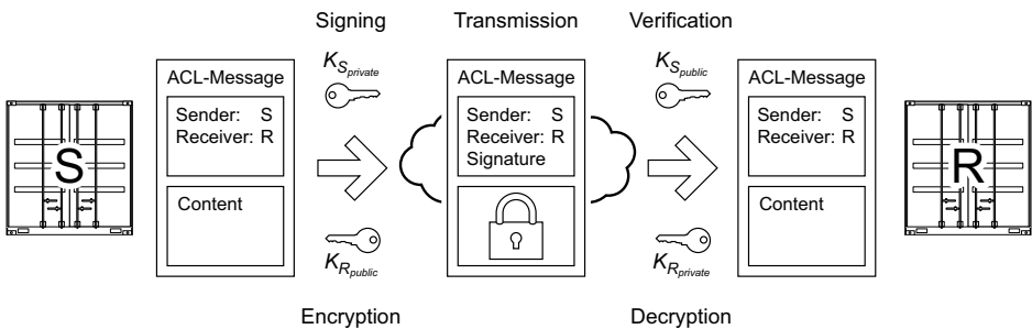
Figure 2: The software agent managing container S sends a message to the agent of container R . Therefore, S signs and encrypts the content of the message before transmission. The received message is then validated and decrypted by R
