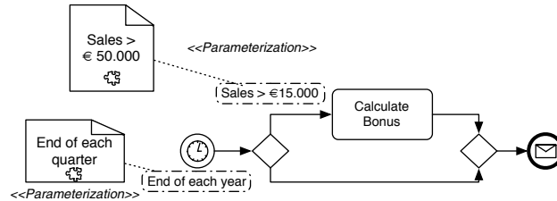
Figure 6. Parameterization in BPMN.
