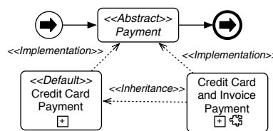
Figure 11. Strategy Pattern in BPMN.
