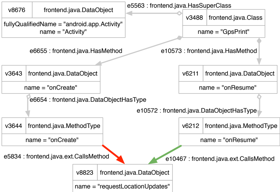
Figure 6: Excerpt of GpsPrint 's TGraph representation (abstract syntax tree).
