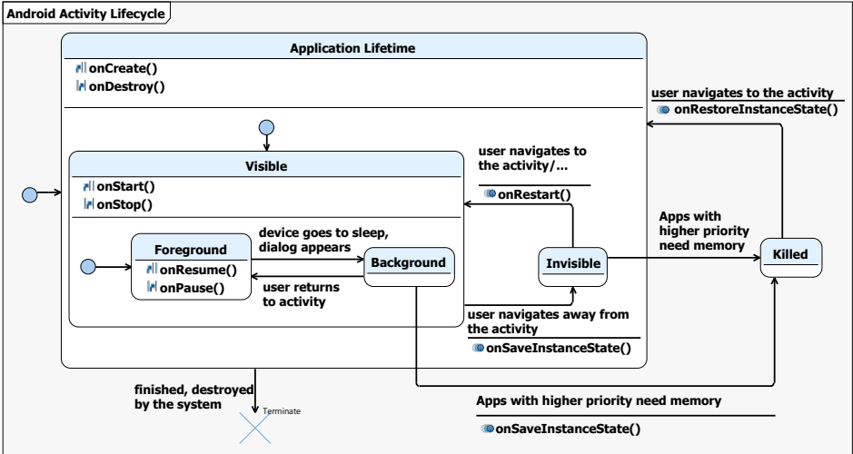
Figure 3: Android State Machine
