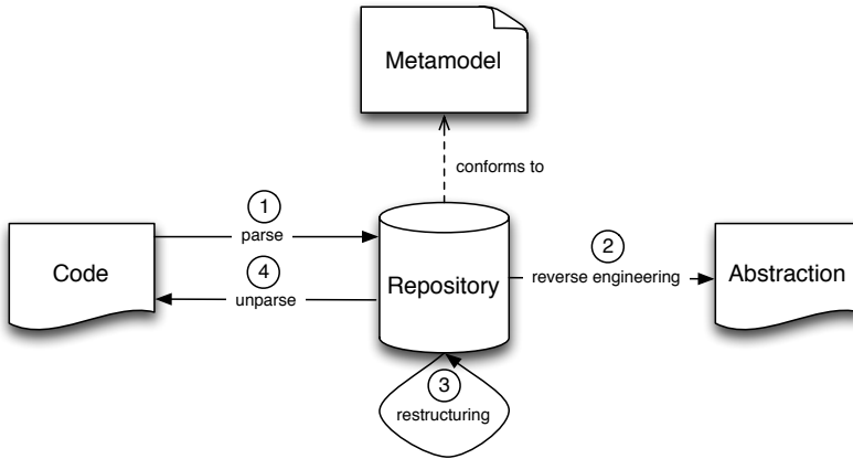
Figure 1: Model based Reengineering Reference Framework
