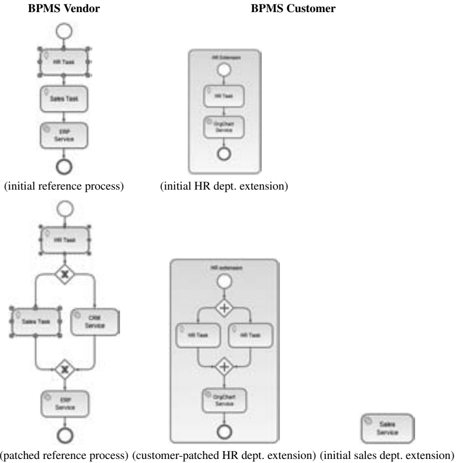
Fig. 1. Extensibility Example
