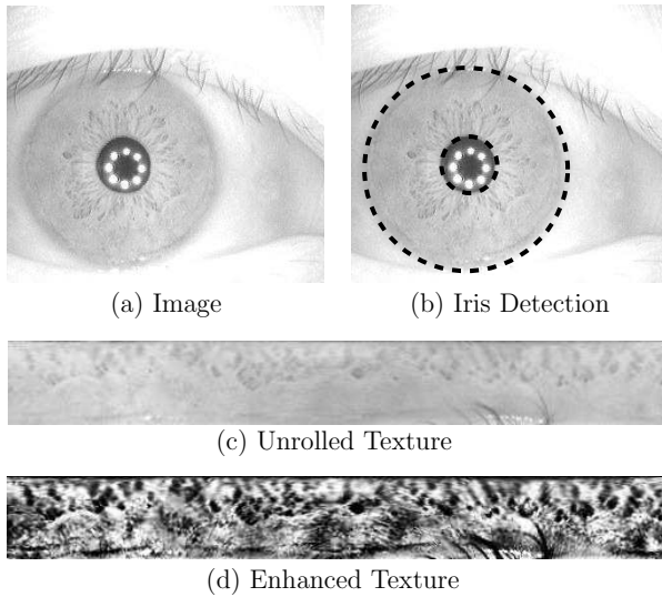
Figure 2: Preprocessing: (a) image of eye (b) detection of pupil and iris (c) unrolled iris texture (d) preprocessed iris texture.
