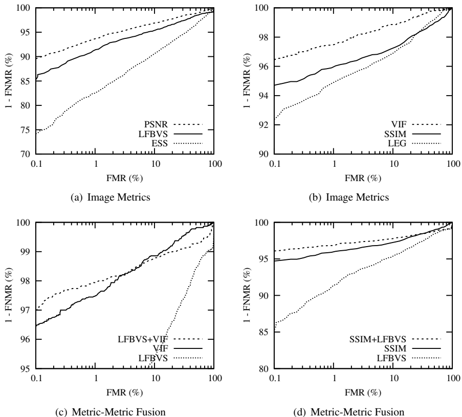
Figure 3: Receiver Operation Characteristic (ROC) curves for image metrics, and selected fusion scenarios of these.
