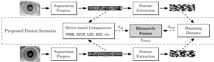
Figure 1: Proposed Fusion Scenario: image quality metric-based scores are combined with Hamming distance-based feature-level scores in order to obtain a final comparison score.
