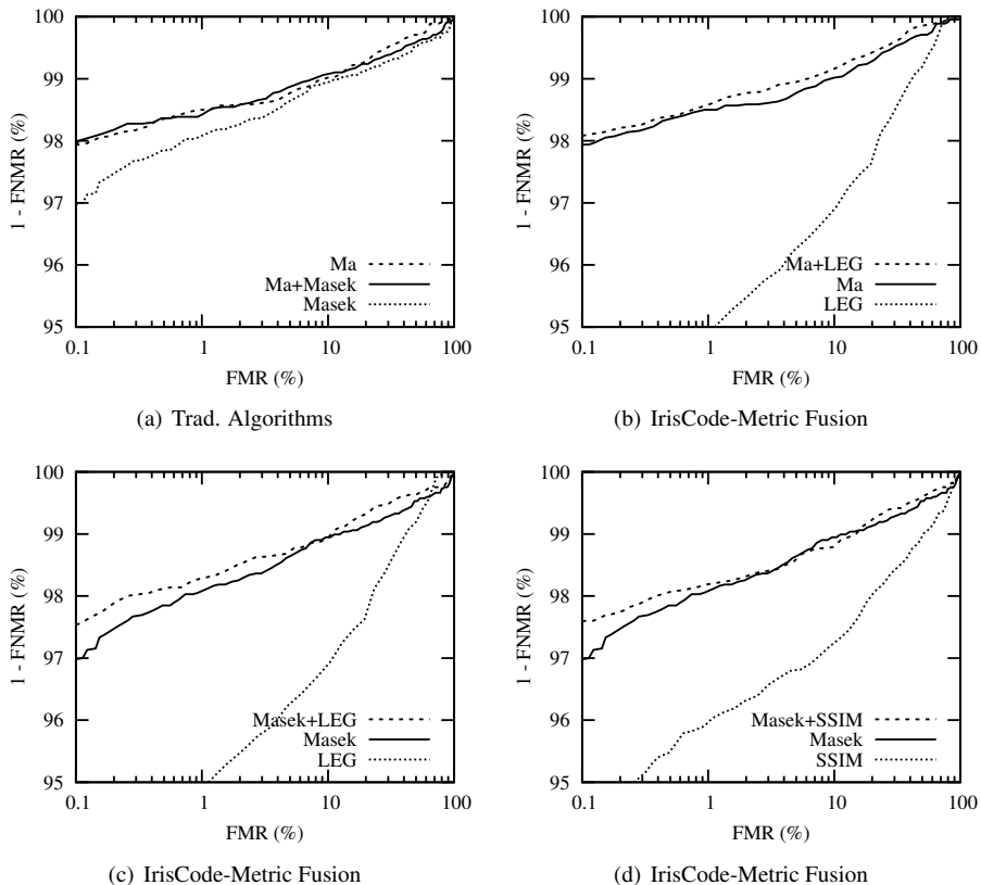
Figure 4: Receiver Operation Characteristic (ROC) curves for traditional algorithms, and selected fusion scenarios of image metrics and these.
