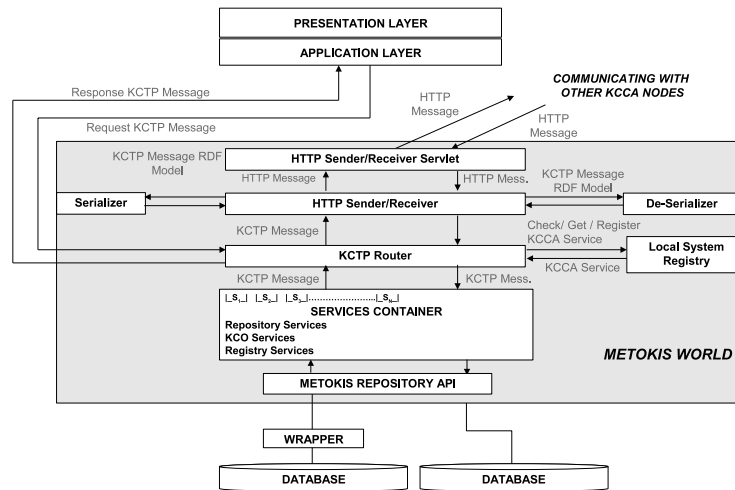
Figure 2: Metokis Architecture
