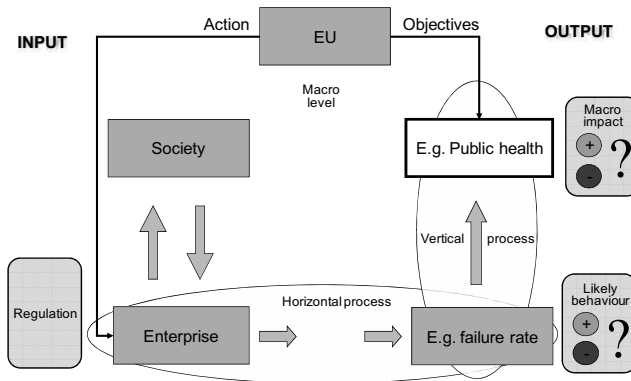
Figure 1 Model overview
