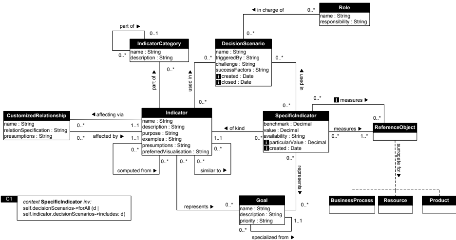
Figure 2 – Excerpt of the SCORE-ML meta model
