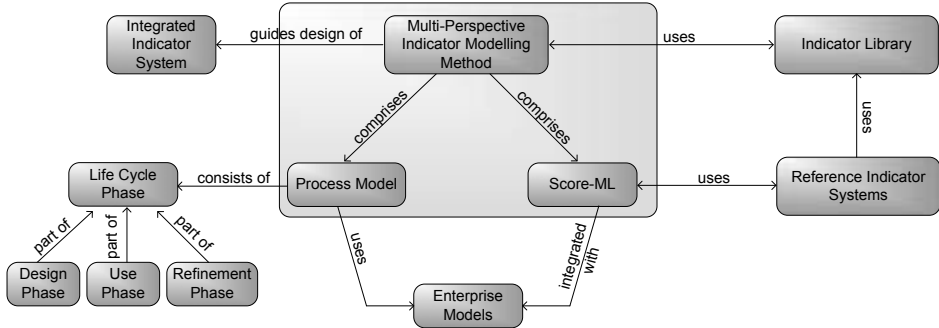
Figure 1 – Elements of the multi-perspective indicator modelling method
