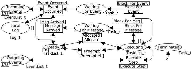
Figure 2: A more detailed view of the behavioral specification of a CPU in the model
