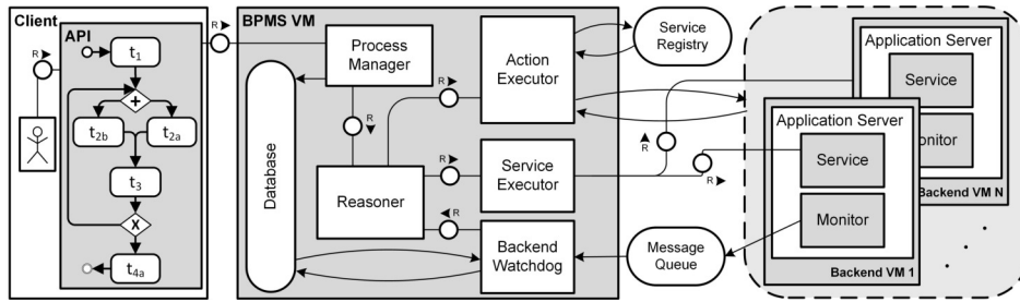
Fig. 1: ViePEP - Architecture
