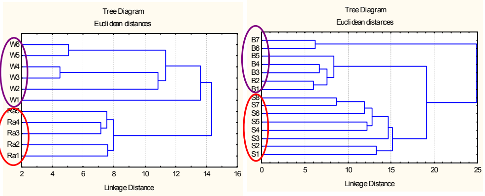
Figure 1: Dendrogram presenting clusters of rainfall and snowfall originated in Racibórz (Ra) and Wrocław (W) (on the left) as well as in Bielawa (B) and Strzelin (S) (on the right)
