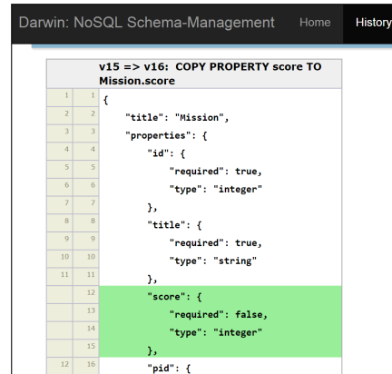
Fig. 2: Darwin screenshot: Schema history.
