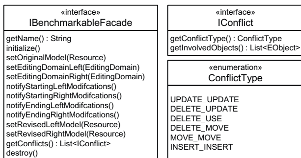
Figure 1: Generic Conflict Detection API
