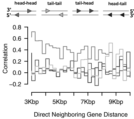
Figure 1: Pearson's correlations for the four promoter pair orientations based on log-ratios of ABI3 ChIP-chip experiments in steps of 250bp within the corresponding gene pair distance interval [3, 10]Kbp. A triangle represents a promoter and the orientation of its tip describes the reading direction of the gene belonging to this promoter.
