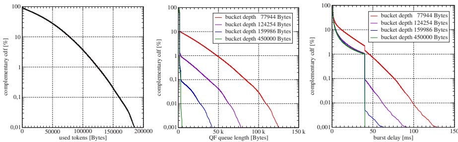
Figure 1: The used tokens from the TBS (l.), the QF queue length (c.) and the burst delay (r.) for a QF aggregate generated by 10 independent on/off sources
