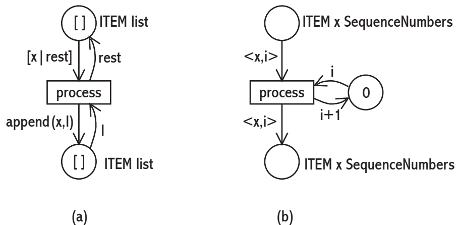
Abbildung 6: Example of streaming activities.
