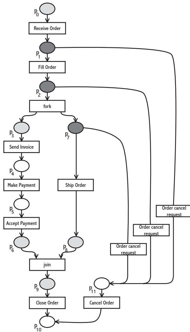
Abbildung 5: Naive Petri-net semantics of the exception example in Figure 3.
