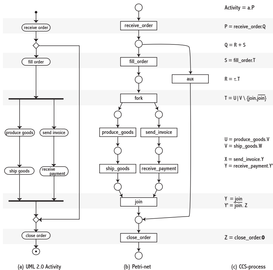
Abbildung 2: Example for the semantic mapping of Fig. 1, and comparison of Petri-nets to CCS as a semantic domain.
