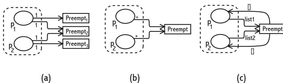
Abbildung 4: Possibilities for preempting a subnet: an individual transition for each marking (a), flush-arcs (b), and high-level nets with list-typed markings (c).
