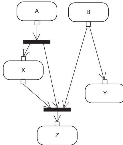
Abbildung 9: Example activity diagram demonstrating the ttc-problem.
