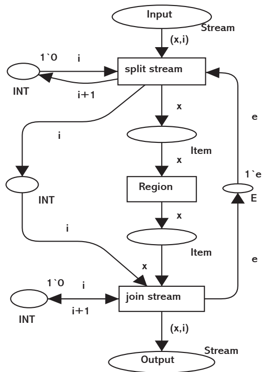
Abbildung 8: A more complex semantical approach to streaming: only a single stream is channeled into the region.
