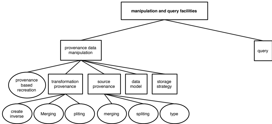
Figure 2: Query and manipulation functionalities
