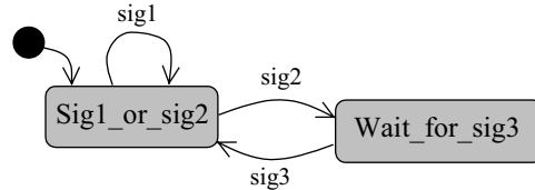
Figure 3. Protocol state machine for MyProtocol
