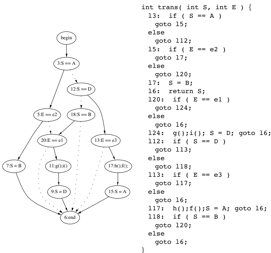
Figure 6: Optimal S-graph with 13 nodes and its implementation in C
