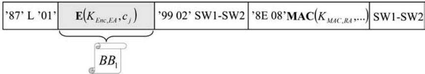
Figure 2: Response APDU containing protected credential c_j
