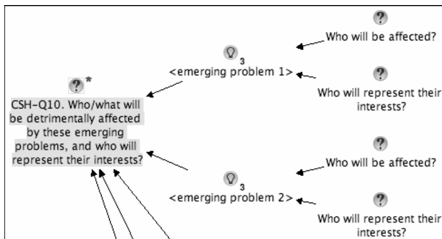
Figure 2: An Issue-template used in Conversational Modelling. For each answer, there are two subsequent Issues.
